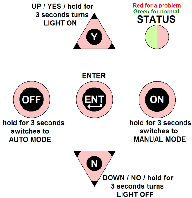
FRONT PANEL LAYOUT
